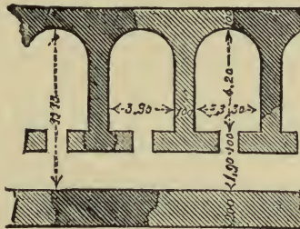
PLAN OF WALL AT BYRSA.
